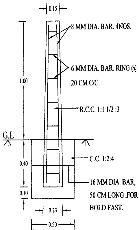
SECTIONAL ELEVATION
