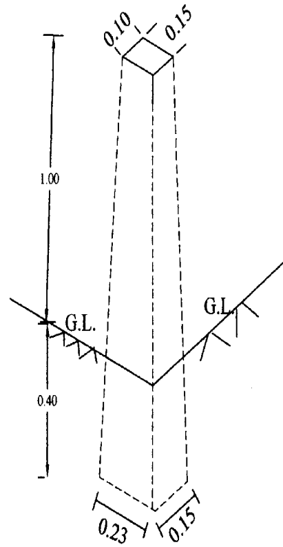
ISOMETRIC VIEW
